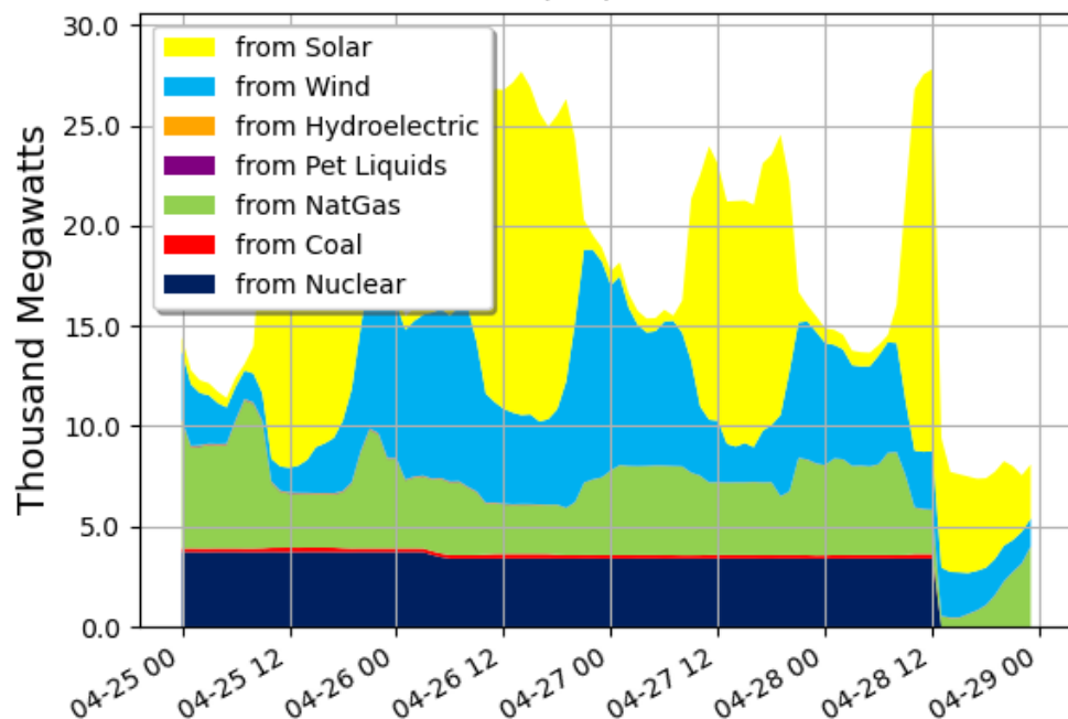
Spain Hourly Electricity Production: 04/25/2025 to 04/30/2025
